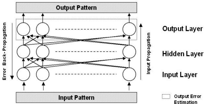
Fig. 2. The Error Back-Propagation Network.
