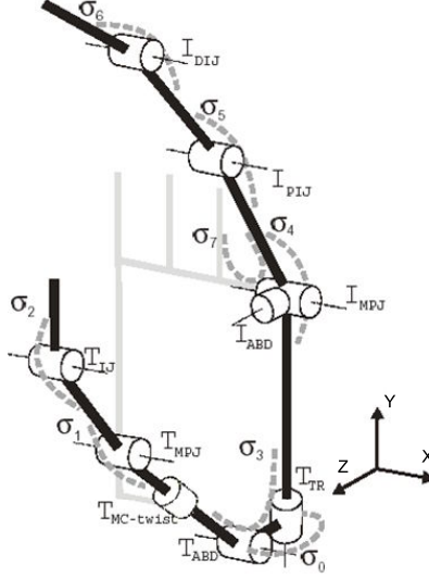
Fig. 1. Kinematic hand model and joint notations
