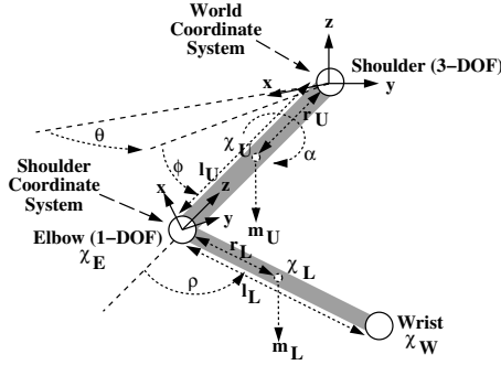
Fig. 3. Articulated Arm Model
