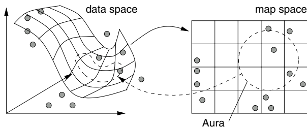
Fig. 4. Illustration of the relation between the AuSOM map space and data space. Neurons within the aura correspond to locations in data space on a 2d-manifold.
