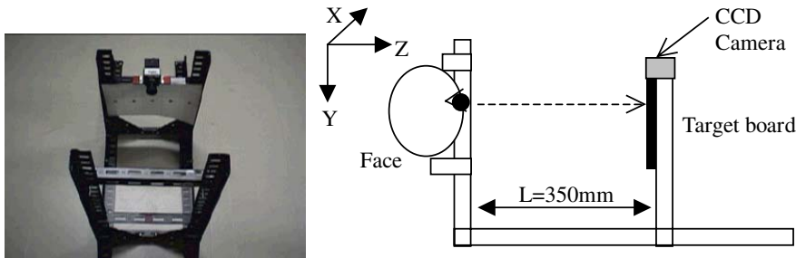
Fig. 6. Calibration device
