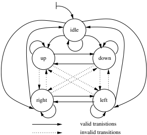
Fig. 4. Overview over the different state transitions in RBA
