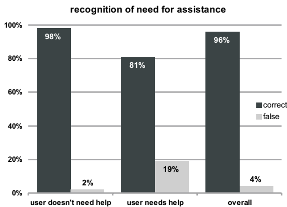
Fig. 8. Recognition rate of the probabilistic neural network used in the first stage of the help system
