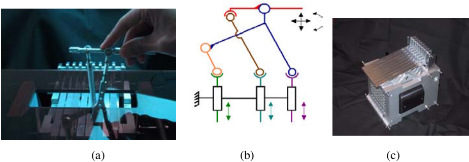
Fig. 2. The 3 degrees of freedom bowing force feedback interface (a) and its cinematic scheme (b) showing the relation between the manipulated part and the 3 parallel actuator (c) The actuator/sensor base shown without the horizontal joystick.
