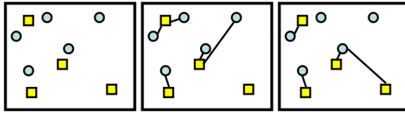
Fig. 2. An example of the chamfer distance. The left image shows two sets of points: a set of circles and a set of squares. The middle image shows a link between each circle and its closest square. The circle-to-square directed chamfer distance is the average distance between a circle and its closest square. The right image shows a link between each square and its closest circle. The square-to-circle chamfer distance is the average distance between a square and its closest circle. The chamfer distance (also known as undirected chamfer distance ) between squares and circles is the sum of the two directed distances.
