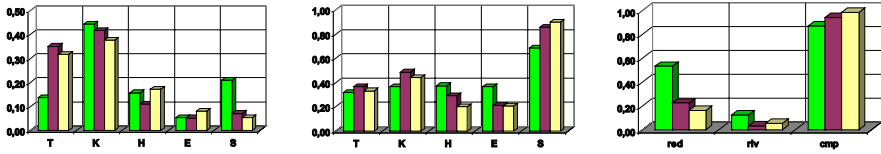
Fig. 3. Distribution of unimodal (left) and multimodal (middle) user interactions with regard to the individual modalities in DVA. The right diagram shows the distribution of multimodal information parts (red=redundant, riv=rivaling, cmp=complementary) in DVA. Concerning each diagram, the left column (green) stands for beginners, the middle column (purple) for normal users and the right column (yellow) for experts
