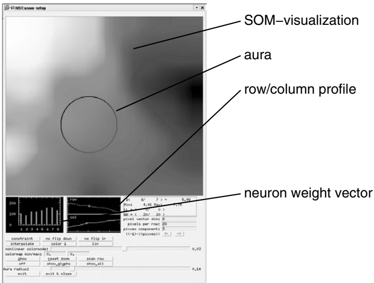
Fig. 5. Visualization of the SOM with Neo/NST [14]. The visualization shows attribute 3 (petal width) of the Iris dataset using a color mapping.
