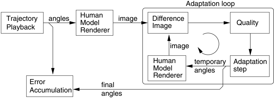
Fig. 3. Signal flow diagram to illustrate the testing environment. For each step of the presented trajectory, the “Adaptation loop”-algorithm tries to adapt the internal model to the input by analyzing the difference image.
